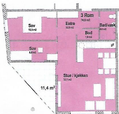
Leilighet B2/B3 - 74,0 kvm.
